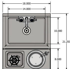
TOP VIEW Scale = 1 : 6
