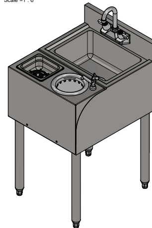
ISO VIEW Scale = 1 : 6
