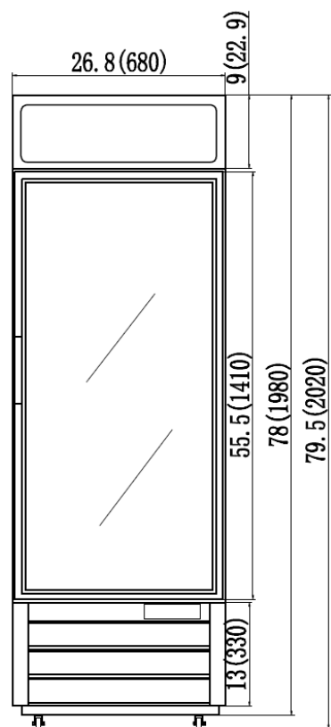
FRONT VIEW
