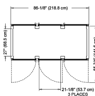
Plan - R/AHT332WP/UT
