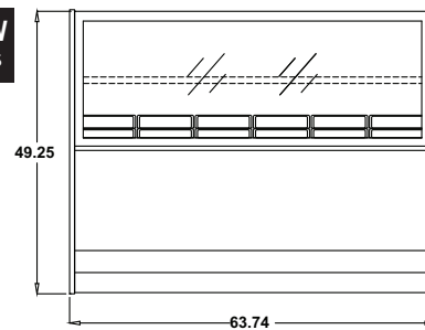
FRONT VIEW 12 Liter pans
