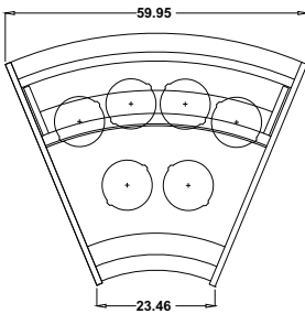
PLAN VIEW Round Tubs
