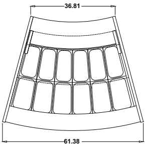
PLAN VIEW 5 Liter pans
