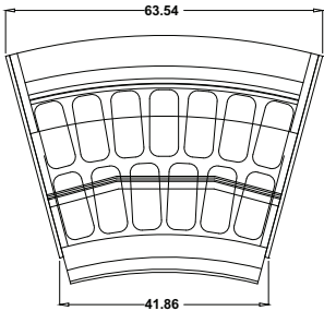
PLAN VIEW 5 Liter pans
