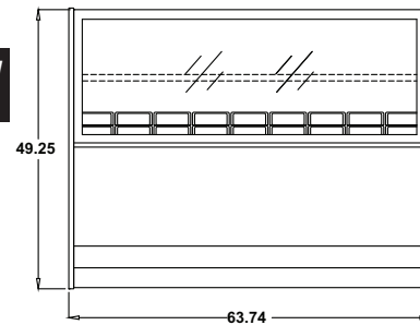
FRONT VIEW 5 Liter pans
