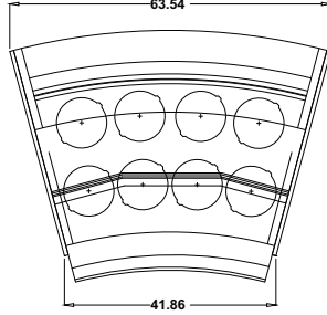
PLAN VIEW Round Tubs
