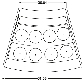
PLAN VIEW Round Tubs
