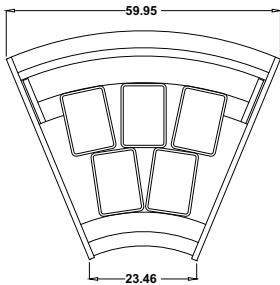
PLAN VIEW 12 Liter pans
