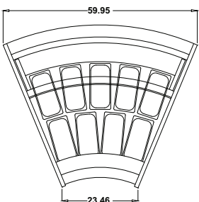
PLAN VIEW 5 Liter pans
