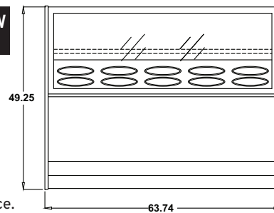
FRONT VIEW Round Tubs
