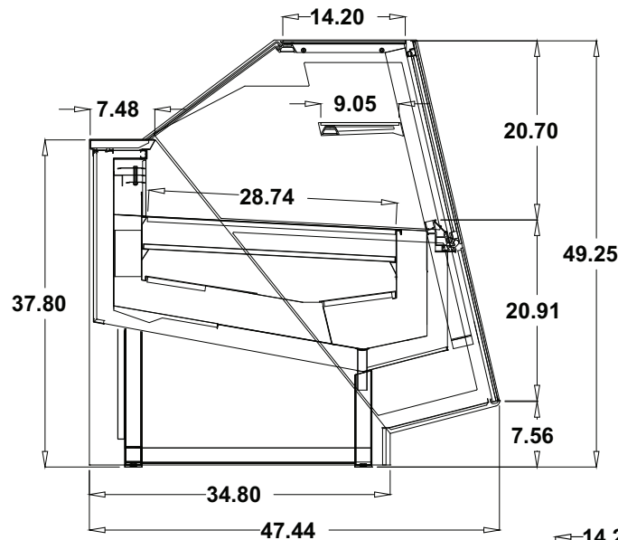
SIDE VIEW 49.25" High
