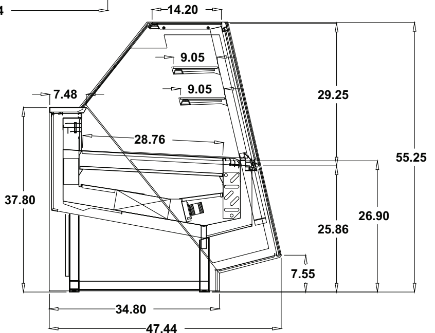
SIDE VIEW 55.25" High
