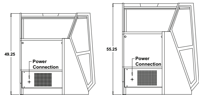
REAR VIEW
