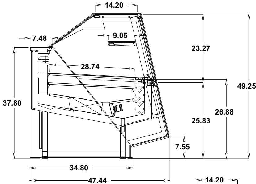
SIDE VIEW 49.25" High
