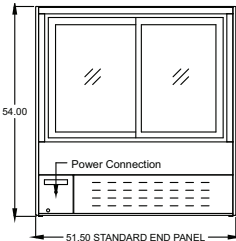
51.50 STANDARD END PANEL
