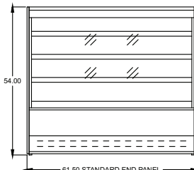
61.50 STANDARD END PANEL
