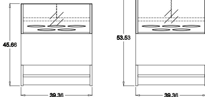
FRONT VIEW (round tubs)
