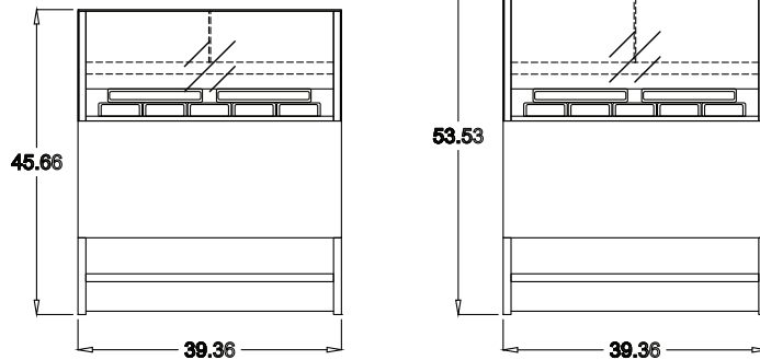
FRONT VIEW (5 liter pans)
