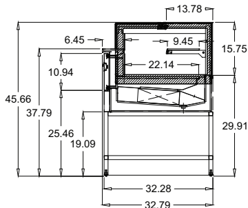
LAR-RVCH40 - 45.66" H
