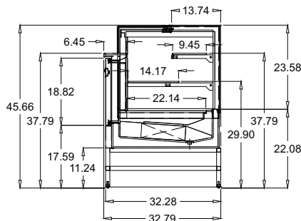
LAR-RVCH40 - 45.66" H
