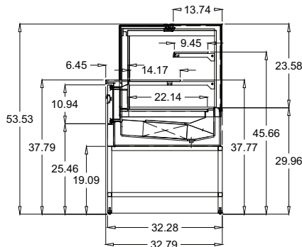
LAR-RVCH40 - 53.33" H
